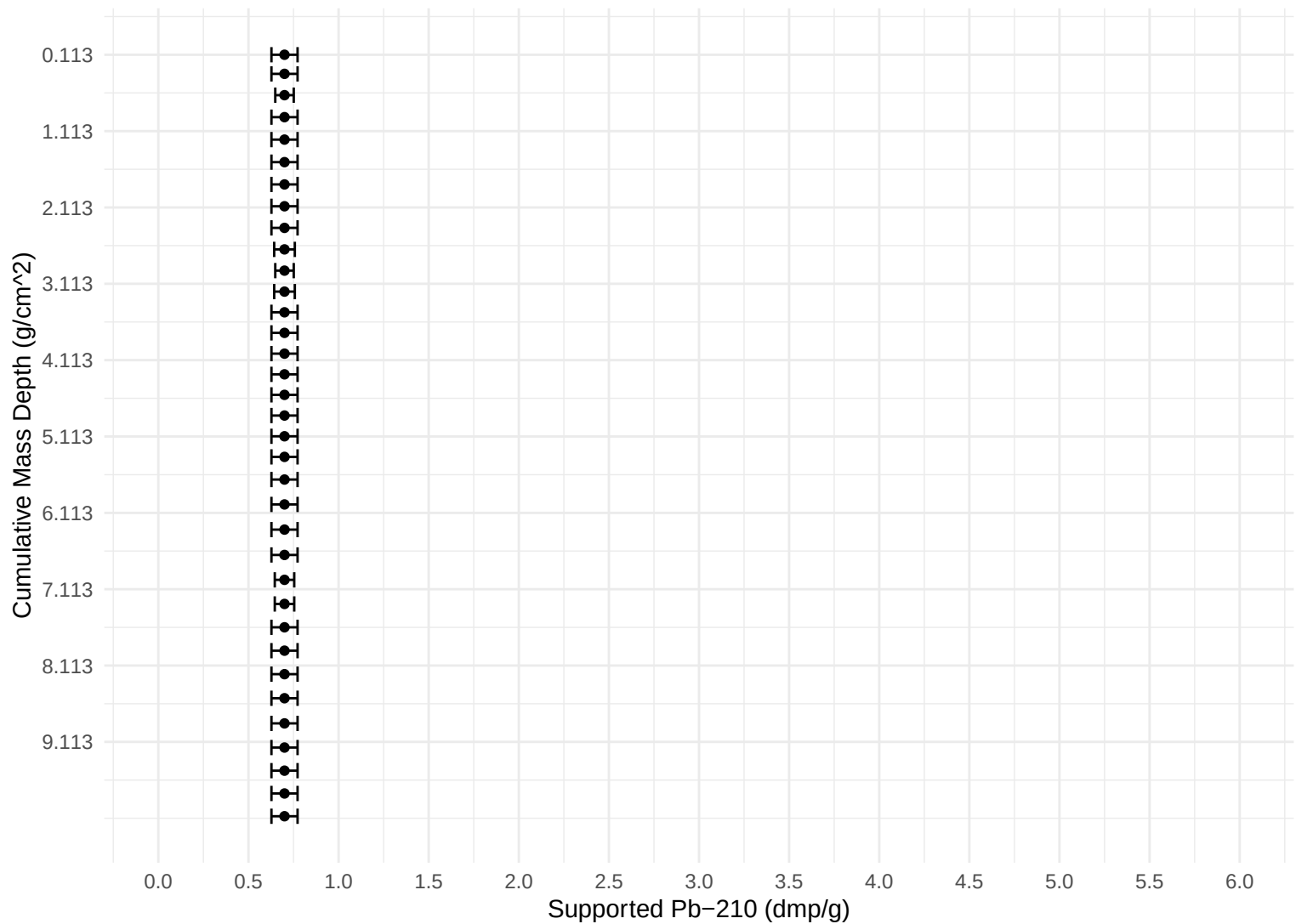
Supported Pb-210 vs Cumulative Mass Depth
